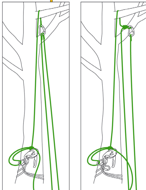
Safety system for double-handled rope clamp and rescue by the ground worker.
