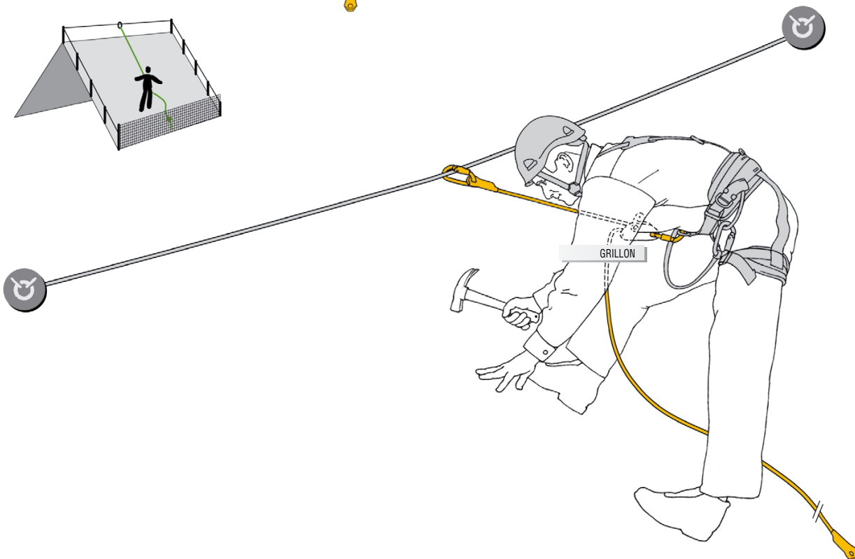
Restraint system for working on steep roofs
